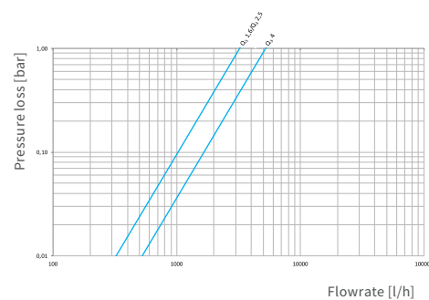
Typical pressure loss curve
